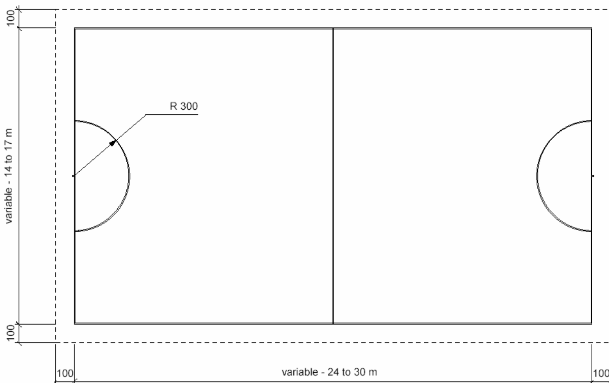
Figure 1 – Recommended dimensions for a reduced-size playing area [cm].
